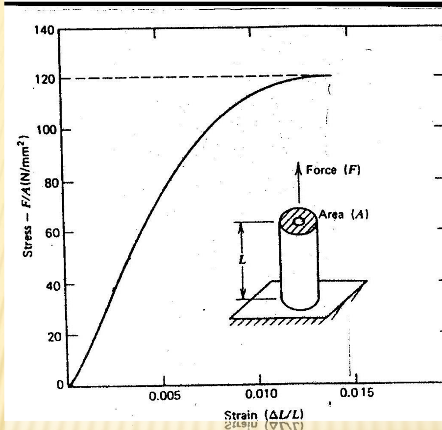
Figure 2. When A Piece Of Bone Placed Under Increasing Tension, Its Strain \Delta L/L Increases Linearly At First (Hooks Law) And Then More Rapidly Just Before It Breaks In Two At 120 \text{ N/Mm}^2 .
