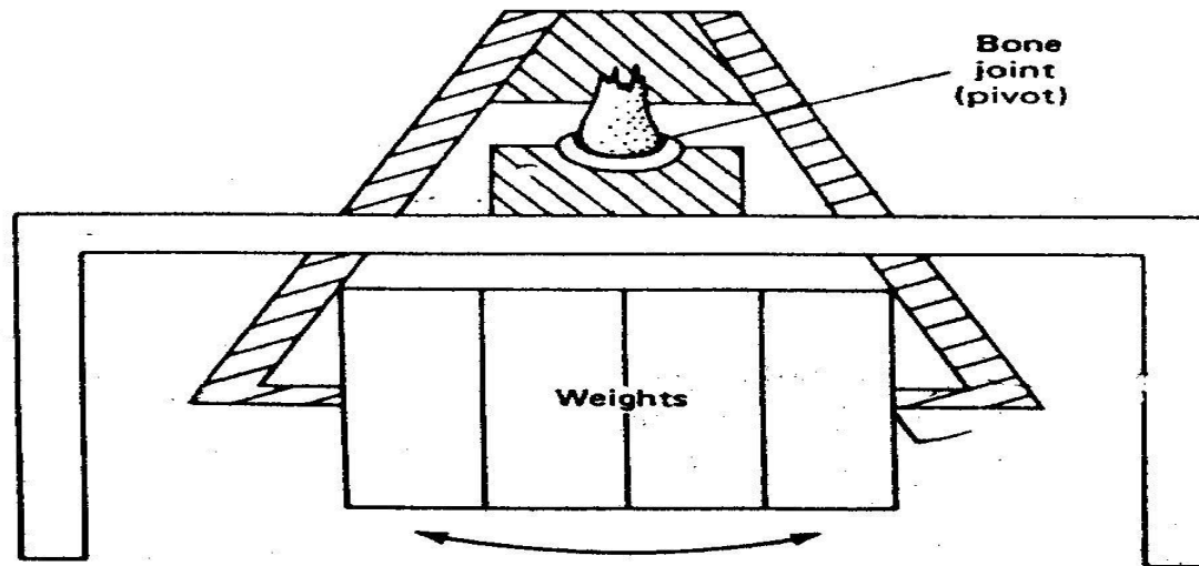
Arrangement for determining the coefficient of friction \mu as the pivot in a pendulum and the decrease in amp with time is measured.
